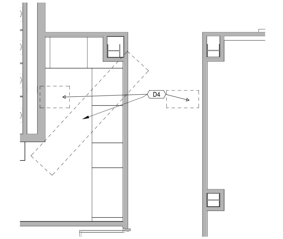
6 Ground Floor Plumbing Demo RCP 1/4" = 1'-0"
