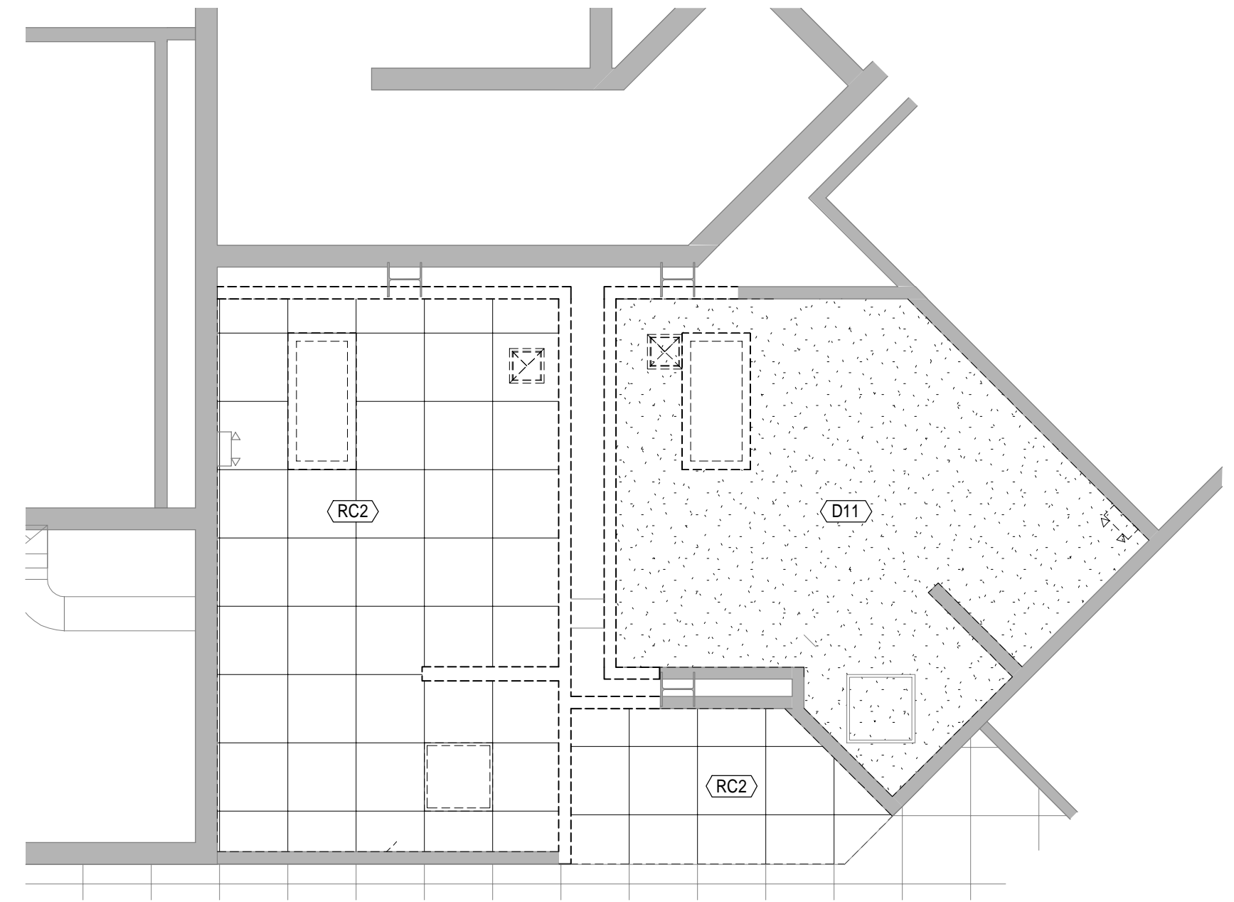
4 Wellness Area Demo RCP 1/4" = 1'-0"
