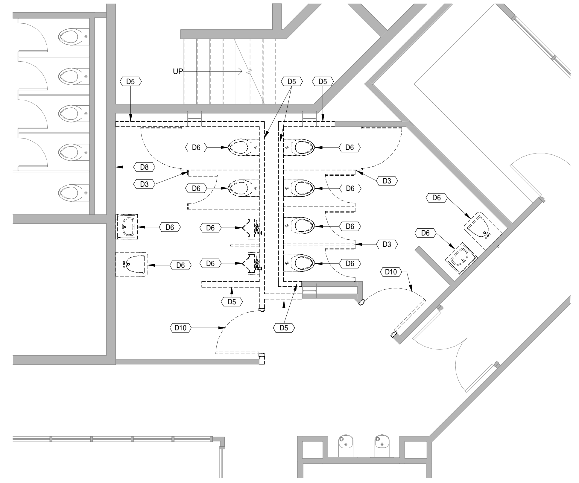
3 Wellness Area Demo Plan 1/4" = 1'-0"
