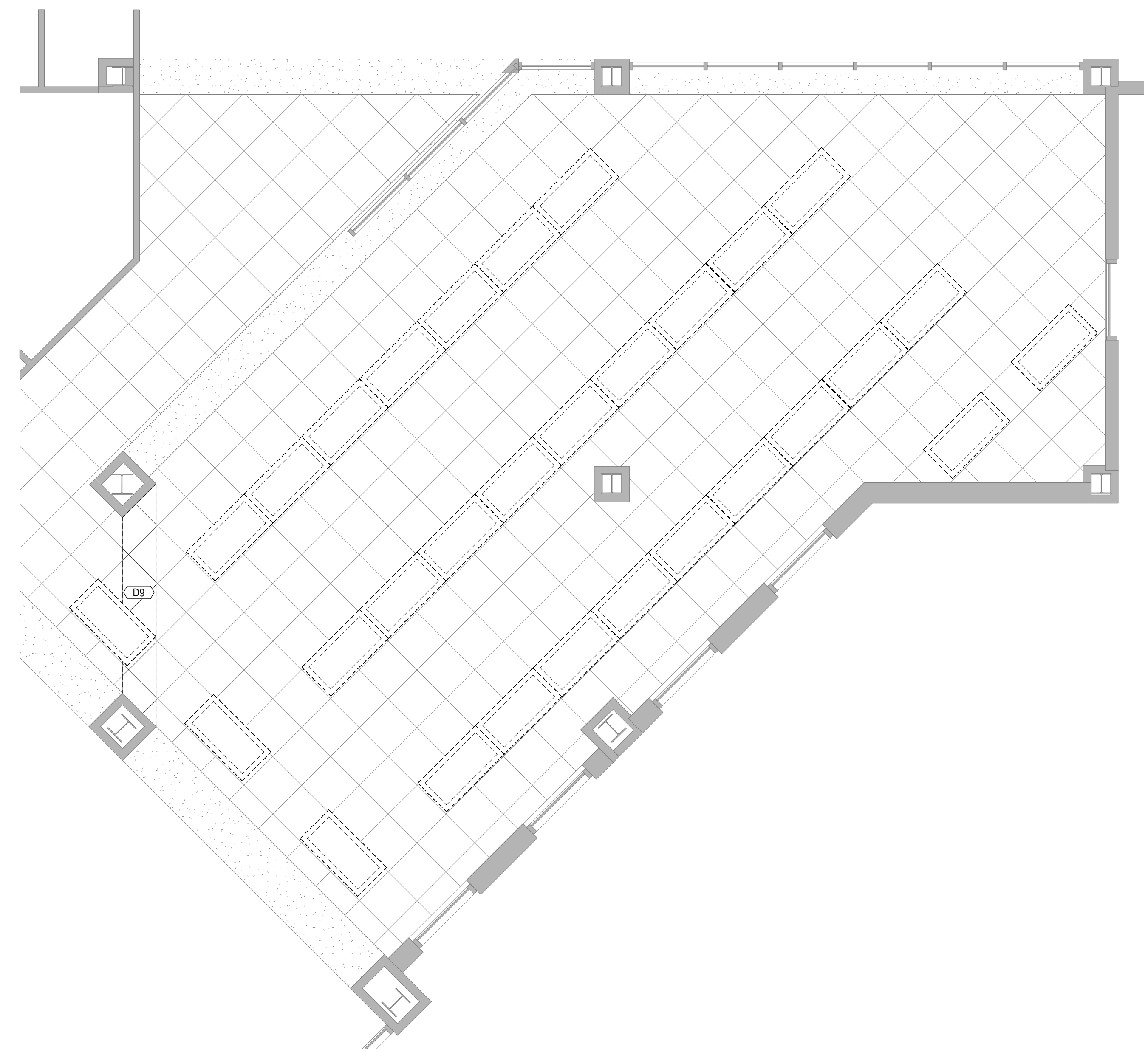
5 Reading Room Demo RCP 1/4" = 1'-0"
