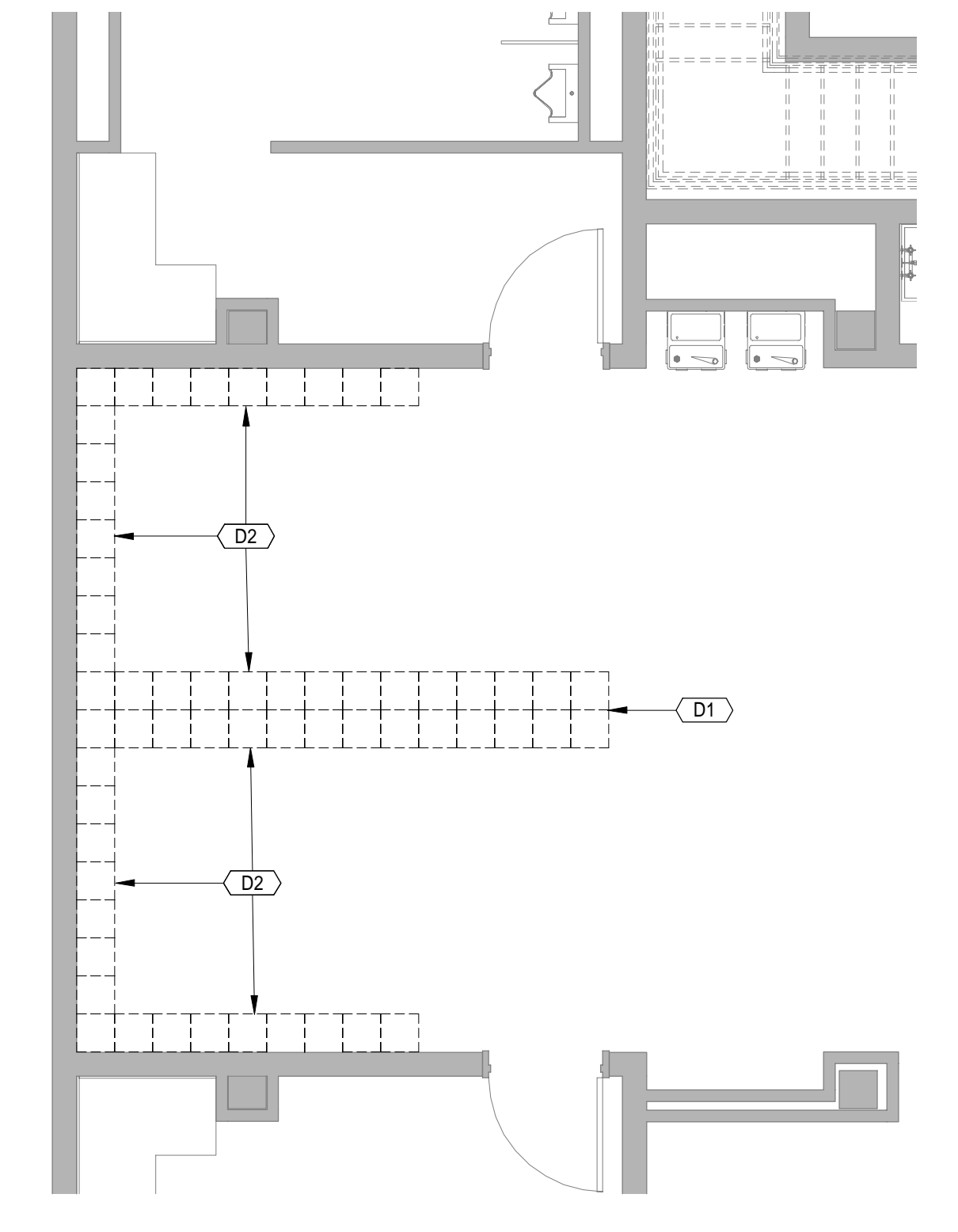
1 Nurse Storage Demo Plan 1/4" = 1'-0"
